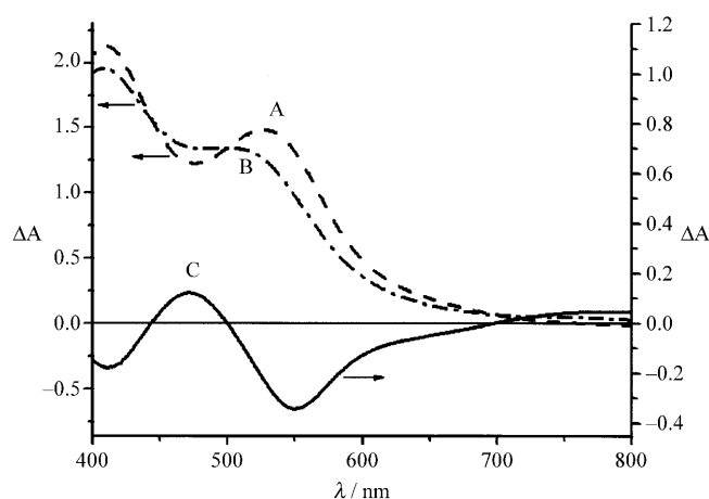
Figure 5. The absorption spectra of CYC-B6S -sensitized TiO 2 electrode (12 μm thick): before (A) and after (B) applying a potential of 1.11 V (versus Ag/Ag + ); C) absorption change after applying potential.
